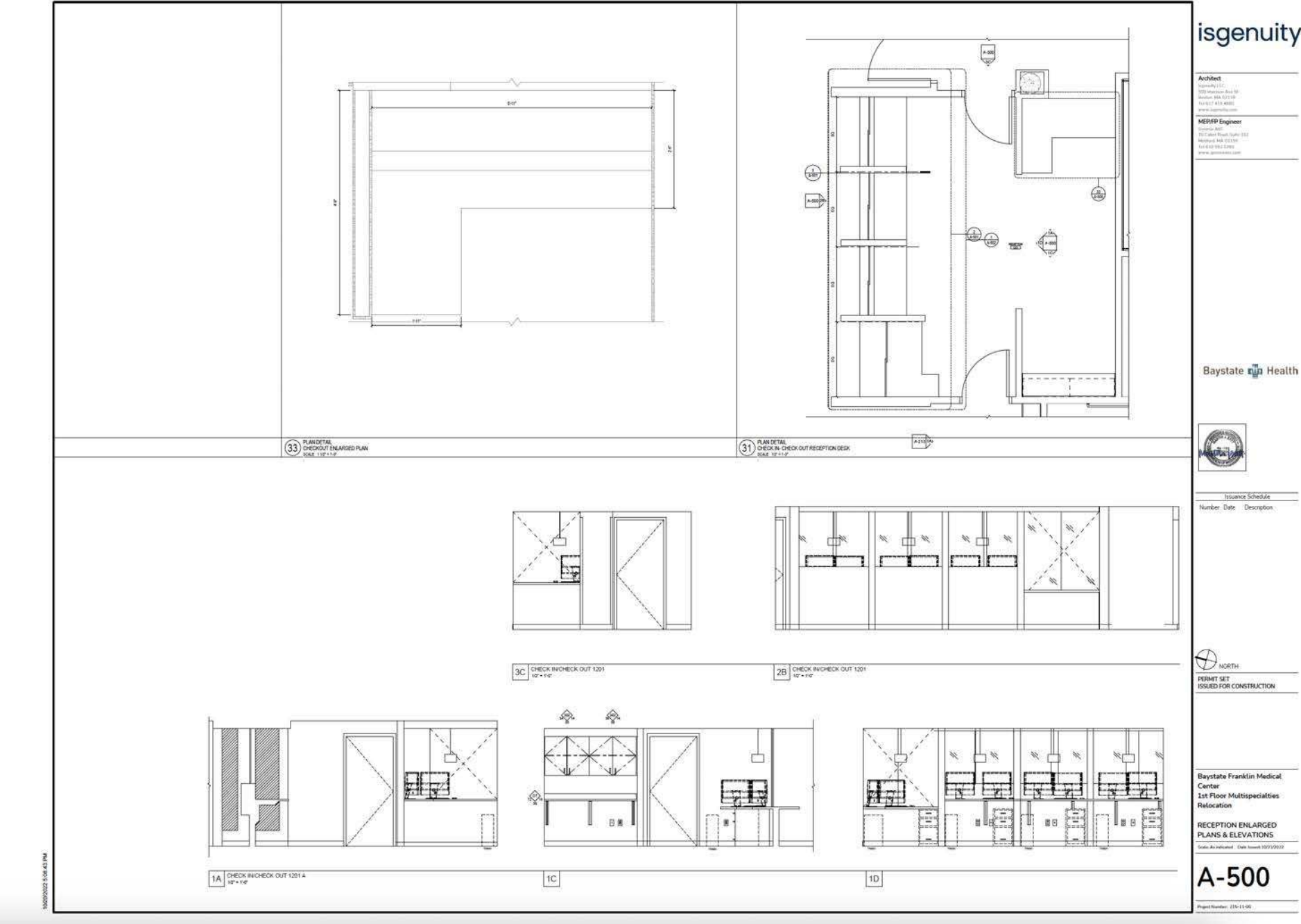
A500 | INTERIOR DETAILS
